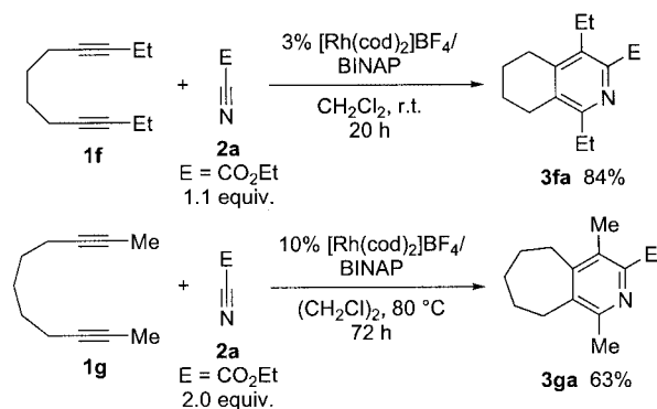
Scheme 1. Rhodium-catalyzed [2+2+2] cycloaddition of 1,7- and 1,8-diynes with ethyl cyanoformate.
