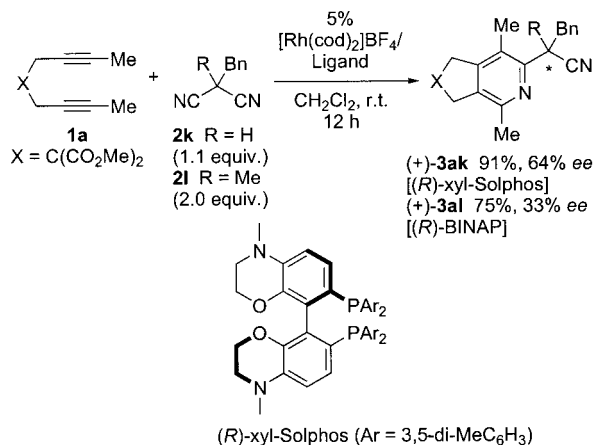
Scheme 6. Rhodium-catalyzed enantioselective [2+2+2] cycloaddition of a 1,6-diyne with substituted malononitriles.
