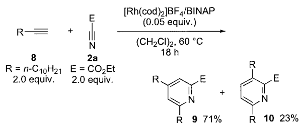
Scheme 5. Rhodium-catalyzed regioselective [2+2+2] cycloaddition of 1-dodecyne with ethyl cyanformate.
