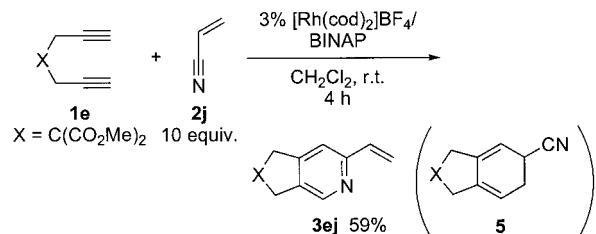
Scheme 3. Rhodium-catalyzed chemoselective [2+2+2] cycloaddition of a 1,6-diyne with acrylonitrile.
