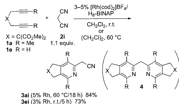
Scheme 2. Rhodium-catalyzed chemoselective [2+2+2] cycloaddition of 1,6-diynes with malononitrile.
