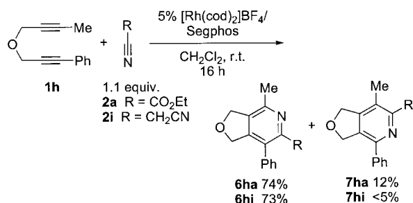
Scheme 4. Rhodium-catalyzed regioselective [2+2+2] cycloaddition of an unsymmetrical 1,6-diyne with nitriles.
